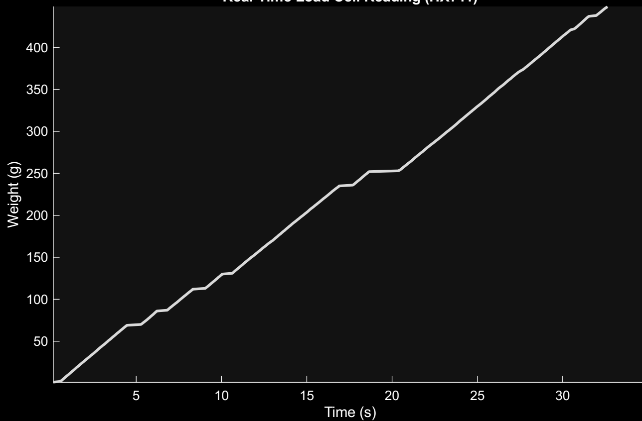
Real-Time Load Cell Reading (HX711)
